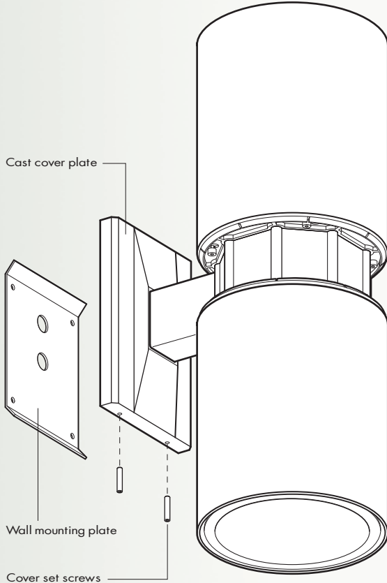
UP/DOWN CYLINDER
