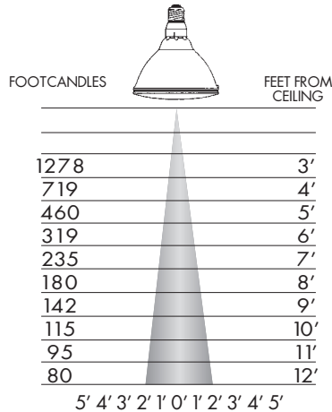
90 WATT PAR38 SPOT BEAM ANGLE = 15°
