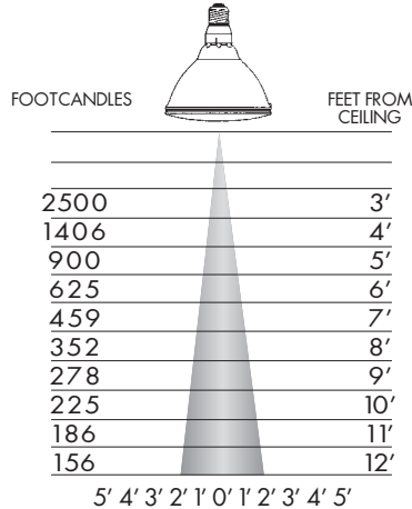
120 WATT PAR38 SPOT BEAM ANGLE = 10°
