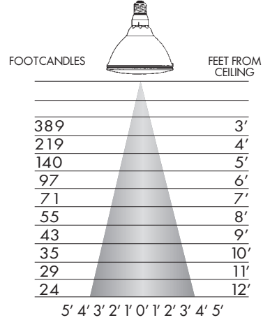
75 WATT PAR38 FLOOD BEAM ANGLE = 30°
