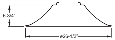
C267 26" x 7" curved hood Total fixture EPA: .94/Weight: 24 Lbs.
