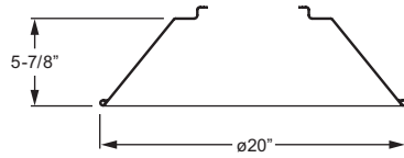
A206 20" x 6" angled hood Total fixture EPA: .84/Weight: 22 Lbs.
