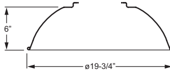
R206 20" x 6" round hood Total fixture EPA: .88/Weight: 22 Lbs.
