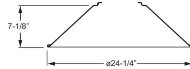
A247 24" x 7" angled hood Total fixture EPA: .95/Weight: 23 Lbs.
