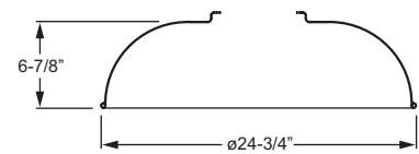
R247 24" x 7" round hood Total fixture EPA: 1.10/Weight: 24 Lbs.
