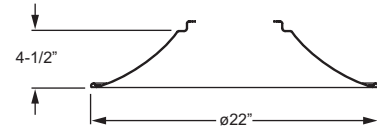
C225 22" x 5" curved hood Total fixture EPA: .80/Weight: 22 Lbs.
