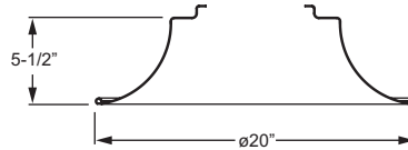
C205 20" x 5" curved hood Total fixture EPA: .83/Weight: 22 Lbs.
