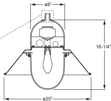
OGL with A206 Hood
