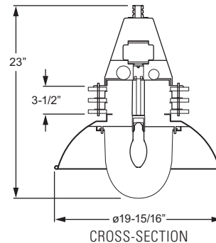
Shown with Opal Bullet Lens and Glow Rings Total fixture EPA: 1.16/Weight: 29 Lbs.
