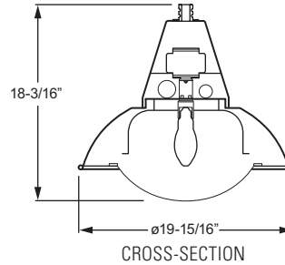
Shown with Clear Drop Polycarbonate Lens Total fixture EPA: .96/Weight: 28 Lbs.
