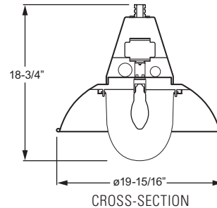
Shown with Opal Bullet Lens Total fixture EPA: .94/Weight: 23 Lbs.
