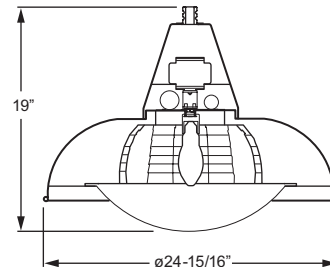
CROSS-SECTION
