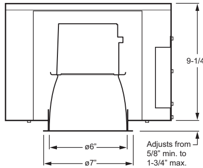
Pan Size: 10-1/4" x 13-3/4" Ceiling Cutout: ø6-1/2"
