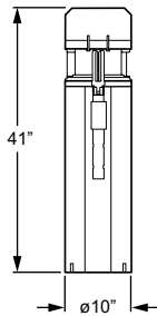
Flat Top (FT) / Vertical Cast Grill (VG) Weight: 194 Lbs.
