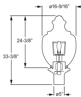
OPA24 shown with Glass Refractor (T3GR or T5GR) Total fixture EPA: 1.40/Weight: 28 Lbs.
