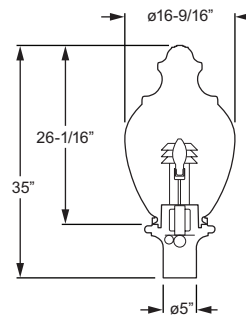
OPA26 shown with Stack Reflector (T5SR) Total fixture EPA: 1.49/Weight: 28 Lbs.
