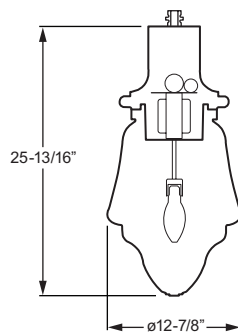
Shown with Bare Lamp (T5BL) Total fixture EPA: .89/Weight: 25 Lbs.
